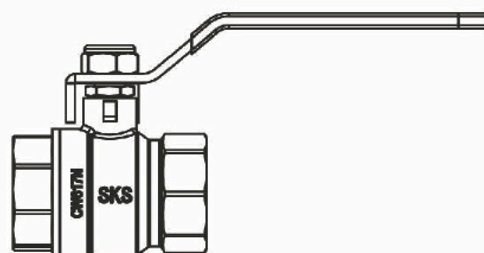
3/4" - 2" Assembly drawing
