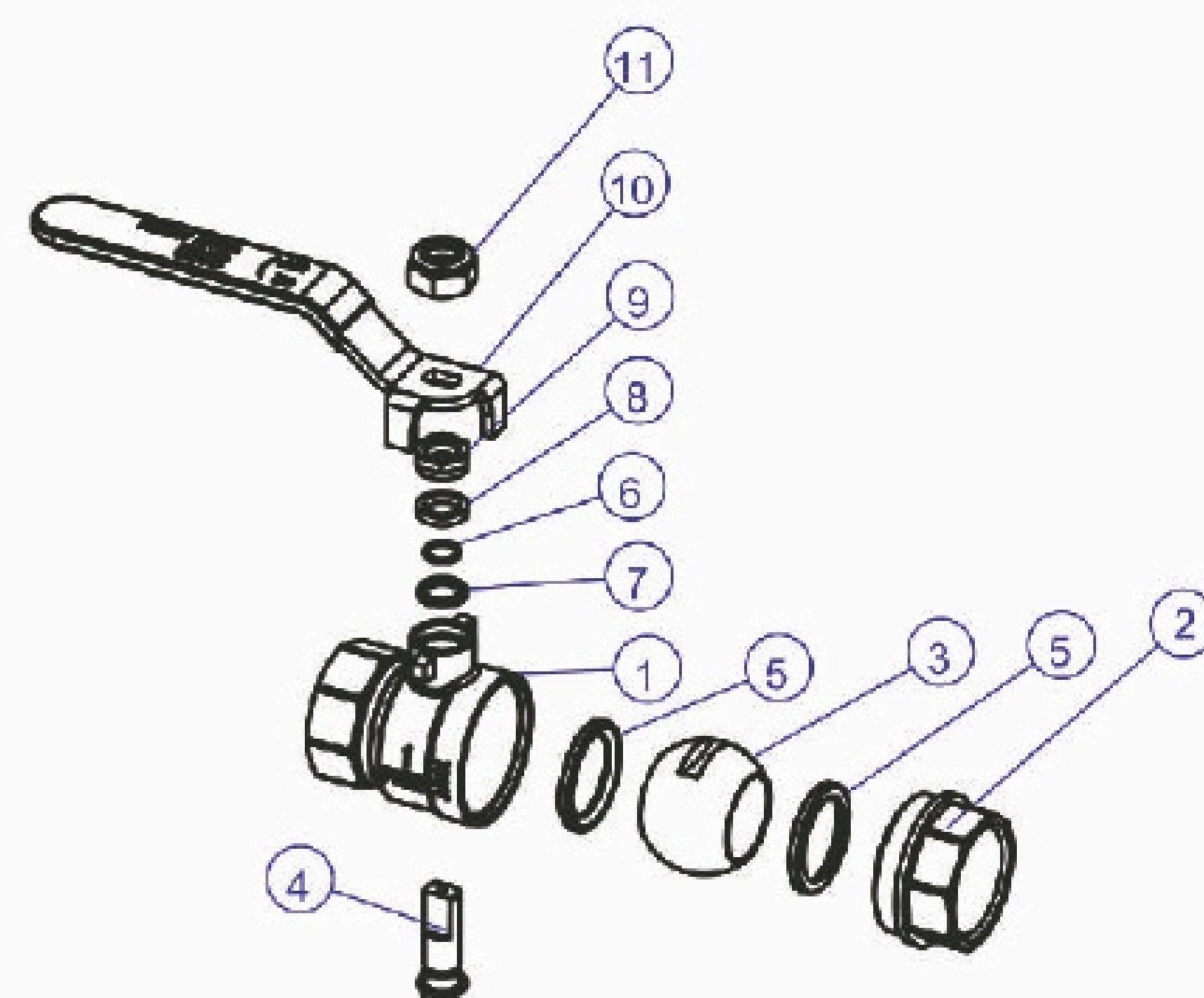
3/4" - 2" Assembly drawing
