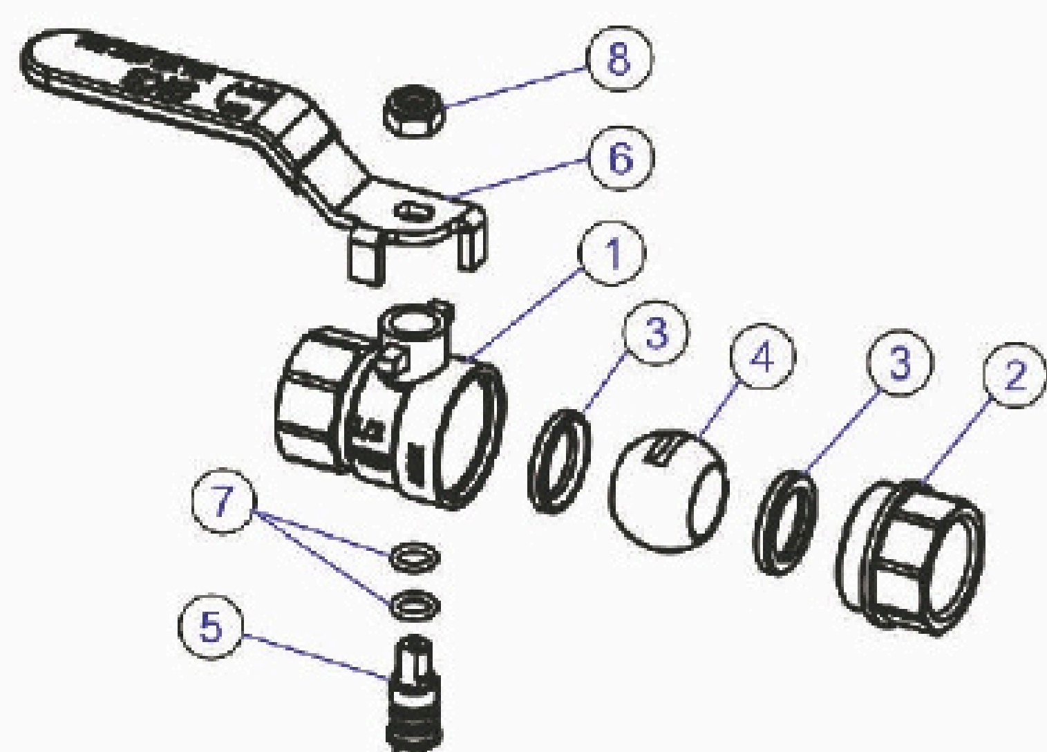
1/4"-1/2" Assembly drawing
